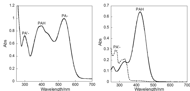
Figure 1. UV-vis spectrum of mPAH 1 in PBS buffer in the dark (left) and that of 2 before and after irradiation. (PAH is the protonated form, PA^- is the deprotonated form of PAH, and PA'^- is the deprotonated cyclized acidic form.)
